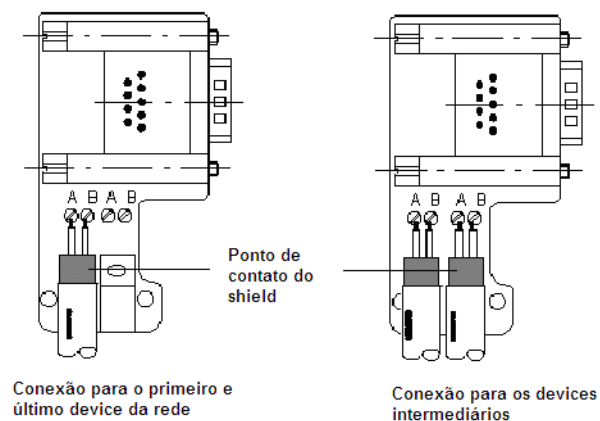
Figura 2 – Conector Profibus-DP DB9.
